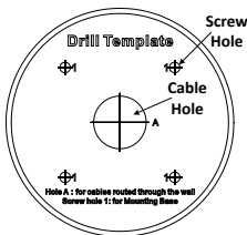
Figure 2-12 Drill Template of the Junction Box
